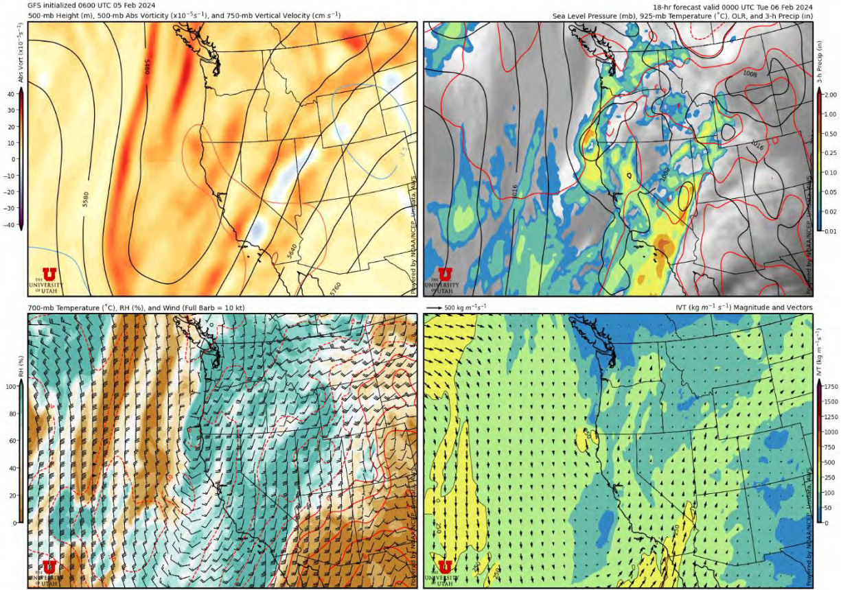
Figure 2.6. GFS (Global Forecast Systems) model forecast (4-panel plot) during a storm event on February 5, 2024.
