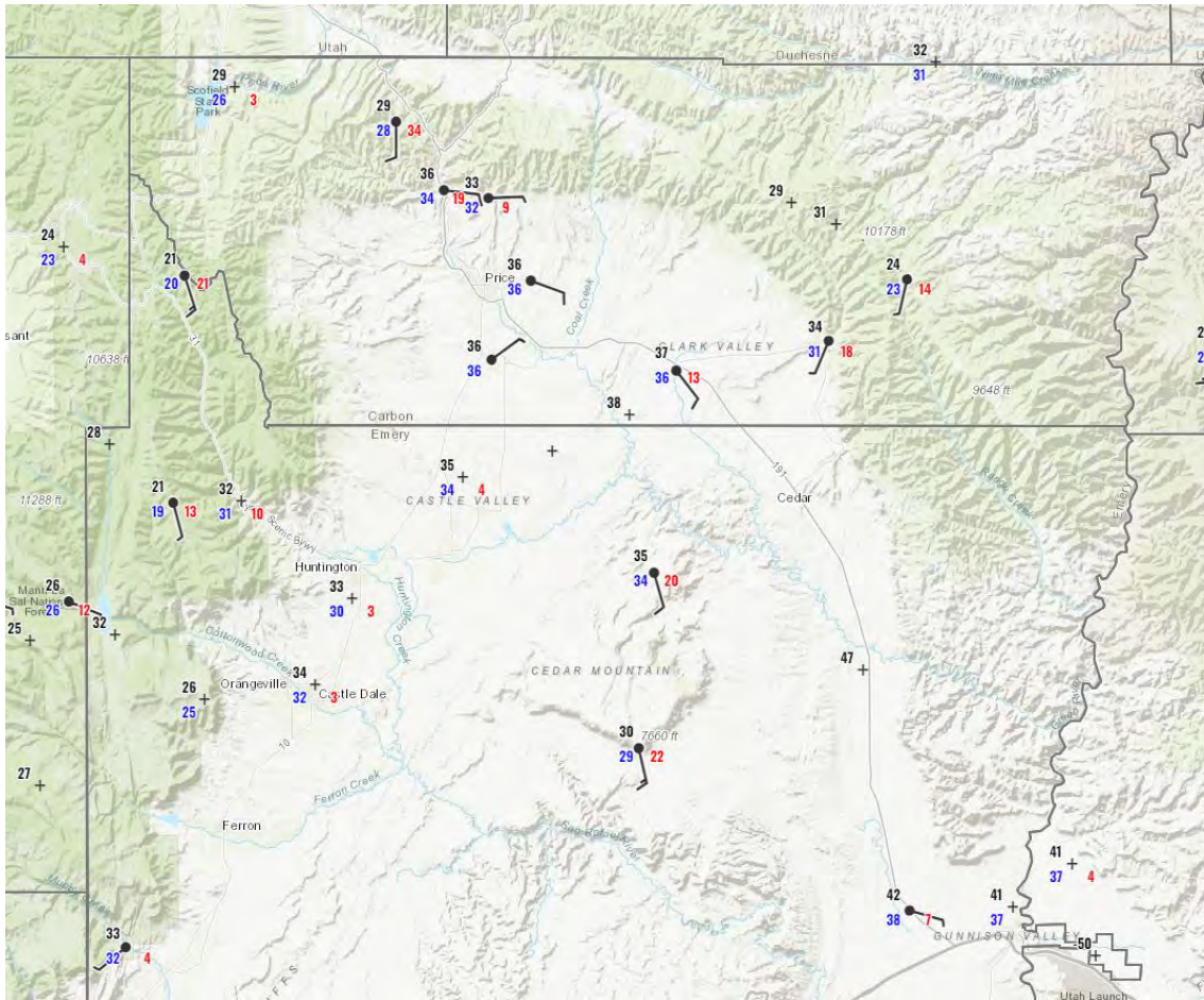
Figure 2.5. MesoWest surface data map from 0500 MST on February 7, 2024. Surface observations are important for diagnosing low level wind patterns, mixing and stability.
