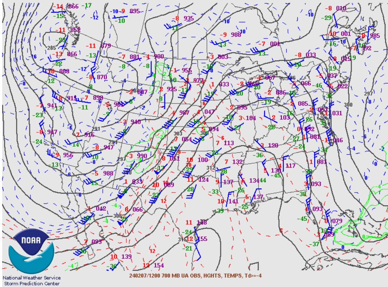
Figure 2.3. 700 mb (approximately 10,000 feet MSL) map valid for 0500 MST (1200 UTC) on February 7, 2024. Among the more notable map features, contours indicate heights (in decameters) of 700 mb pressure level, red numbers are temperature (°C), green numbers are dewpoints (°C), blue lines with barbs/flags represent wind speed and direction.
