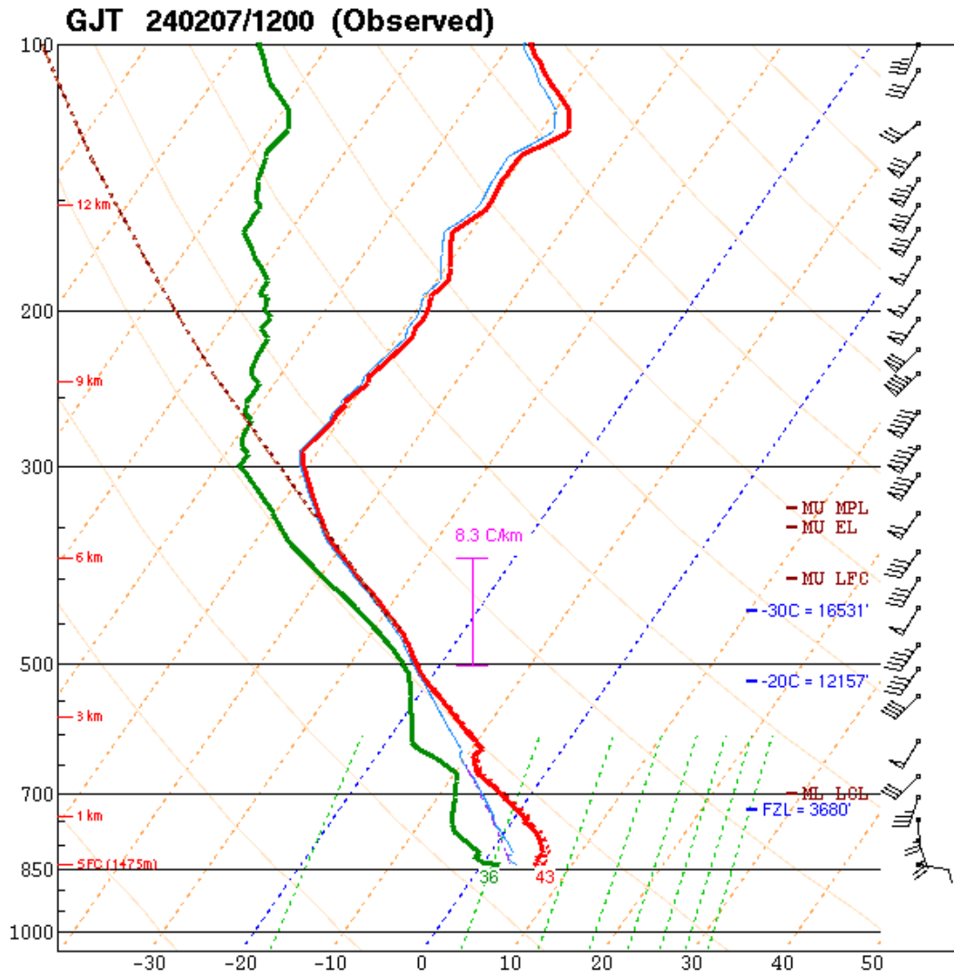
Figure 2.4. Weather balloon/rawinsonde sounding from Grand Junction, CO, valid at 12Z/0500 MST on February 7, 2024, showing temperature (red line), dewpoint (green line) and wind speed/direction (right side barbs) from the surface to 100 mb (approximately 52,000 feet MSL).
